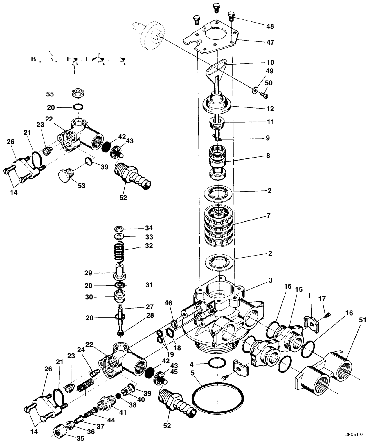
Figure 13: Model 5600 and 5600 E
